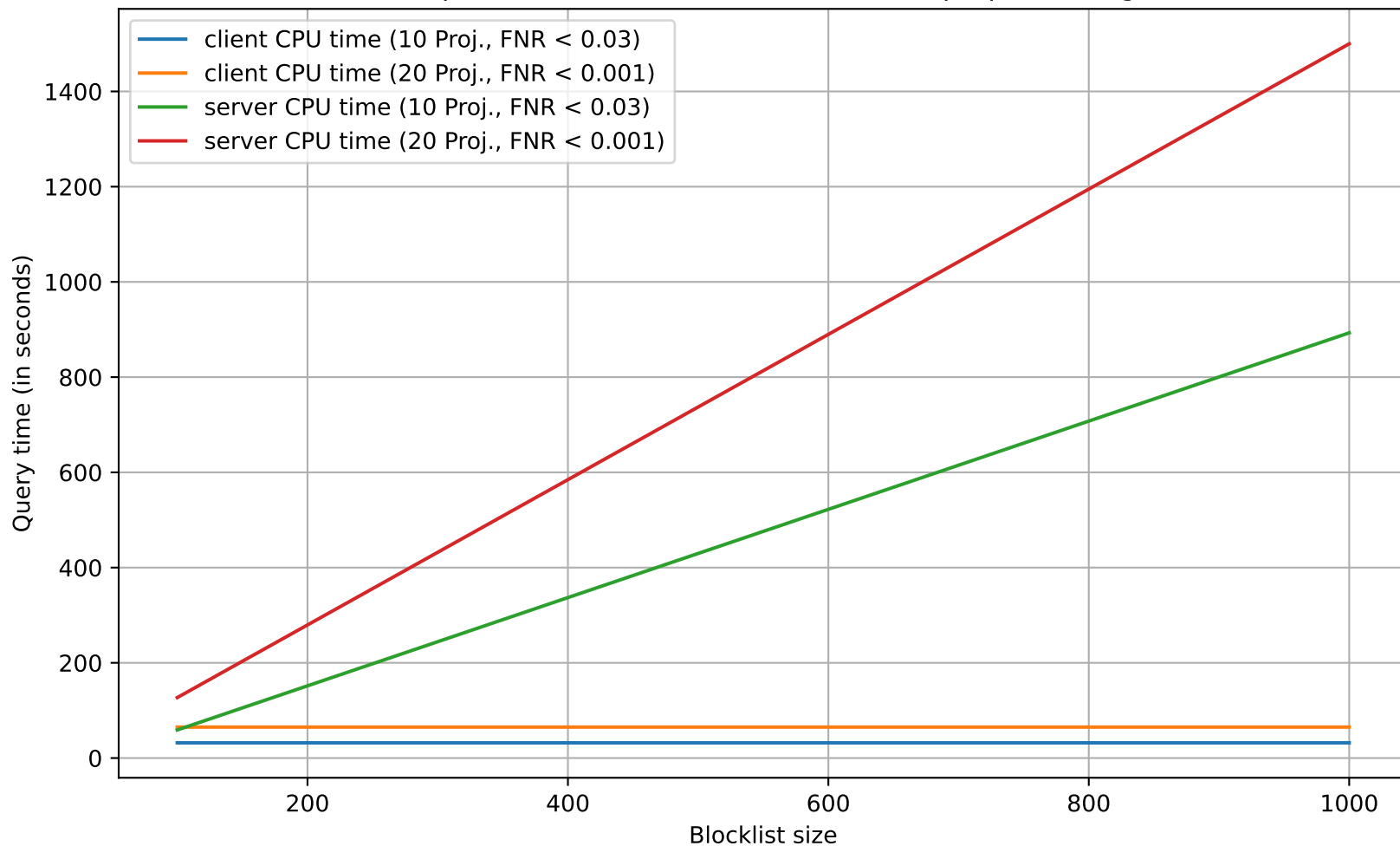
Compute time vs. Blocklist size (with no preprocessing)
